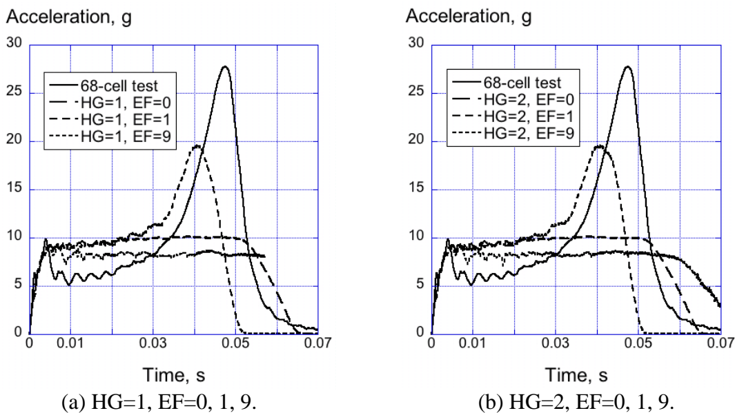
Figure 19. Correlation of the 68-cell DEA with Mat 126 , based on the 104-cell input curves.
