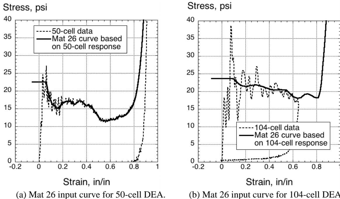
Figure 11. Mat 26 input curves for the 50- and 104-cell DEA components.
