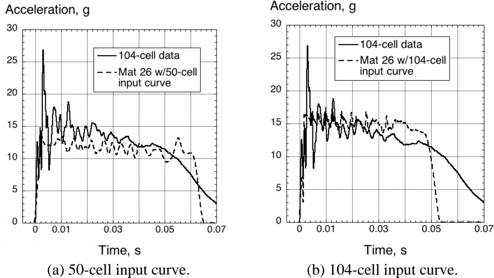
Figure 15. Test-analysis correlation of the 104-cell DEA with Mat 26 material models.
