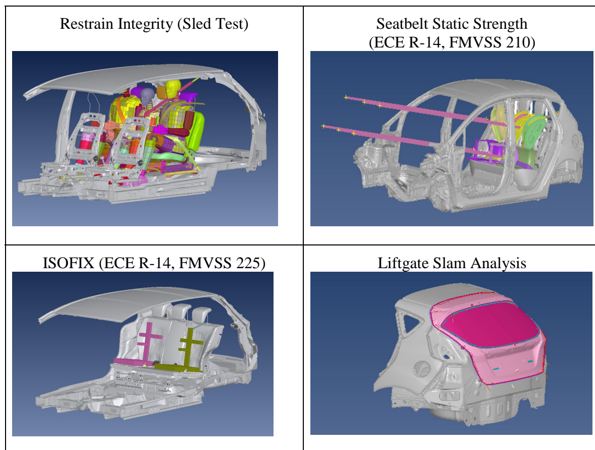
Figure 2. Some of the load case developed to Task Manger Templates
