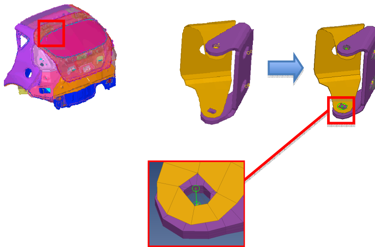
Figure 7. The liftgate hinges connectors are applied and revolute joints are created.
