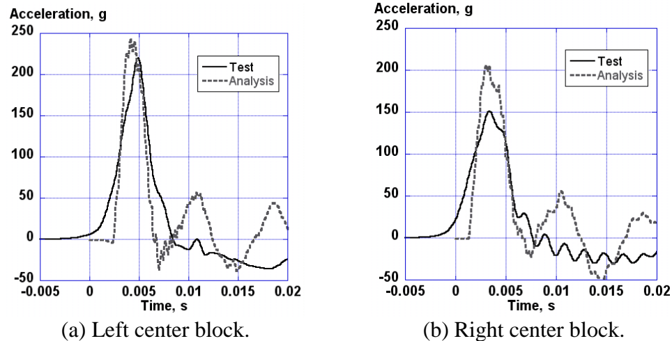
Figure 18. Post-test correlation of 1.5-in. mesh SPH model with 1°-rolled fuselage section.
