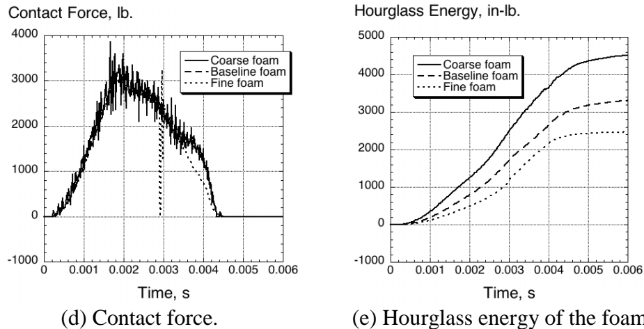
Figure 17. Time-history responses with a constant fine panel mesh and varying foam densities.
