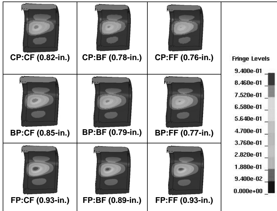
Figure 8. Resultant deflection plots of RCC Panel 6 at 2.8 ms.
