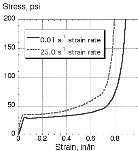
Figure 6. Compressive material properties of BX-250 foam for two different strain rates.
