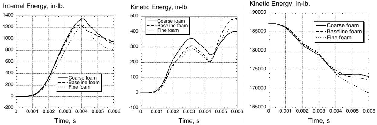
(a) Internal energy of the panel. (b) Kinetic energy of the panel. (c) Kinetic energy of the foam.
