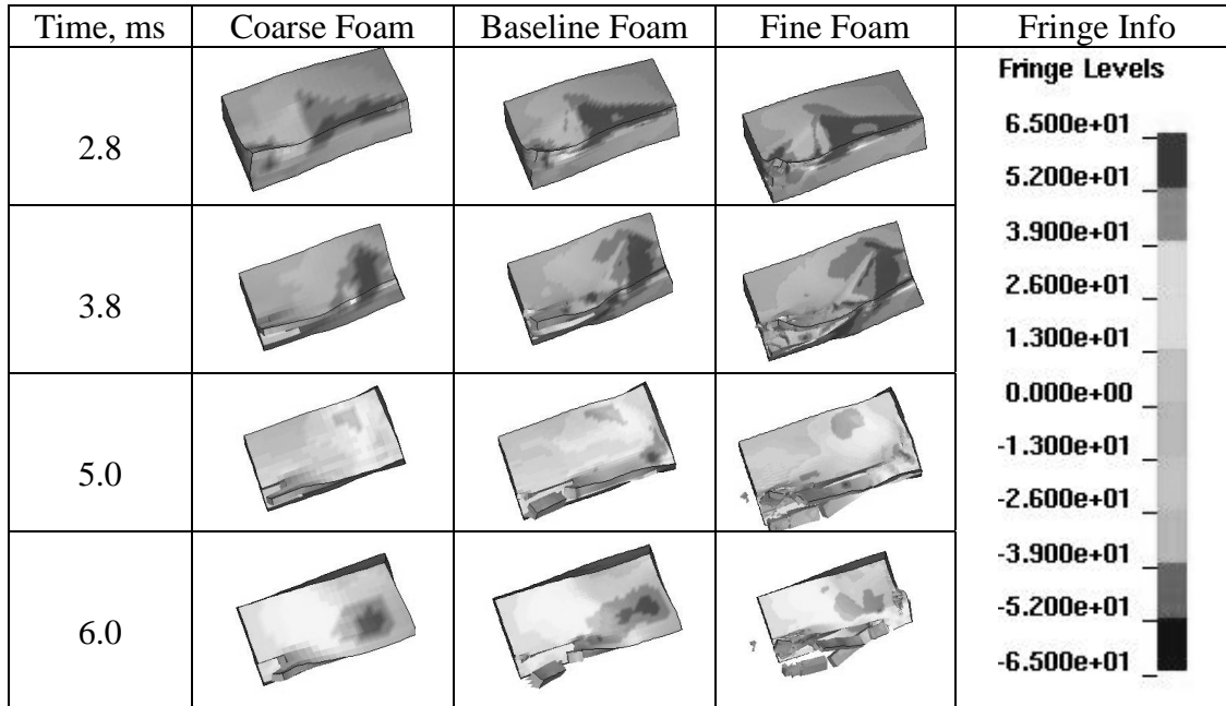
Figure 13. Effective stress fringe plots for varying foam mesh densities and a baseline panel.
