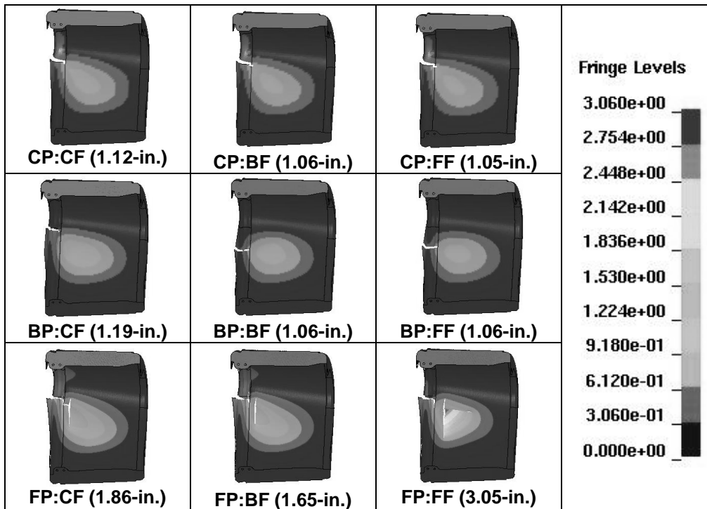
Figure 10. Resultant deflection plots of RCC Panel 6 at 5.0 ms.
