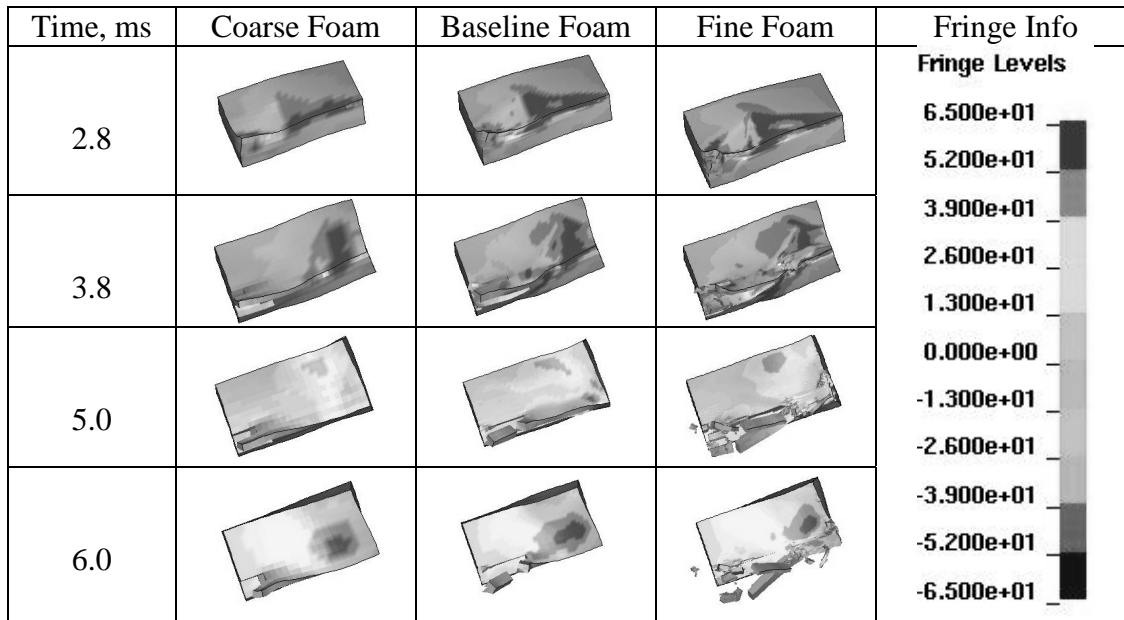
Figure 14. Effective stress fringe plots for varying foam mesh densities and a fine panel mesh.
