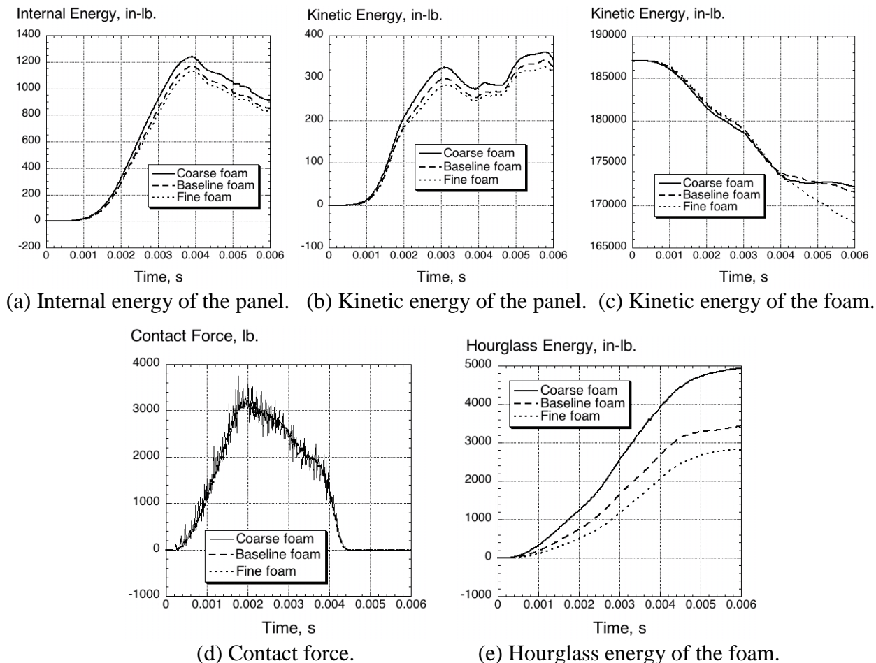
Figure 15. Time-history responses for a constant coarse panel mesh and varying foam densities.
