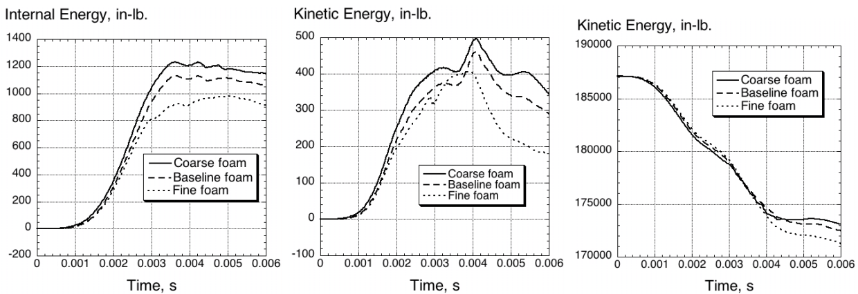
(a) Internal energy of the panel. (b) Kinetic energy of the panel. (c) Kinetic energy of the foam.
