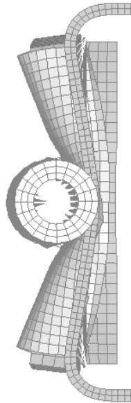
Figure 5. Typical deformation results
