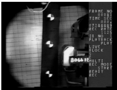
Figure 3. Test setup initial position
