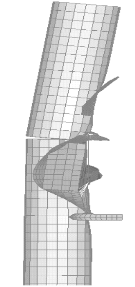
Figure 6. Typical deflection
