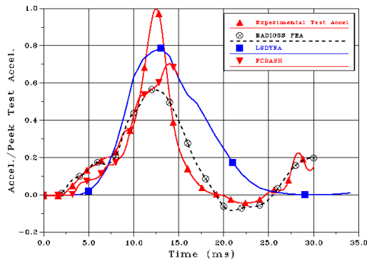
Figure 7 . Tibia Normalized Acceleration
