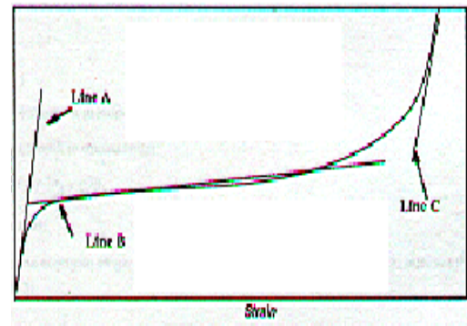
Figure 2b. Typical foam response
