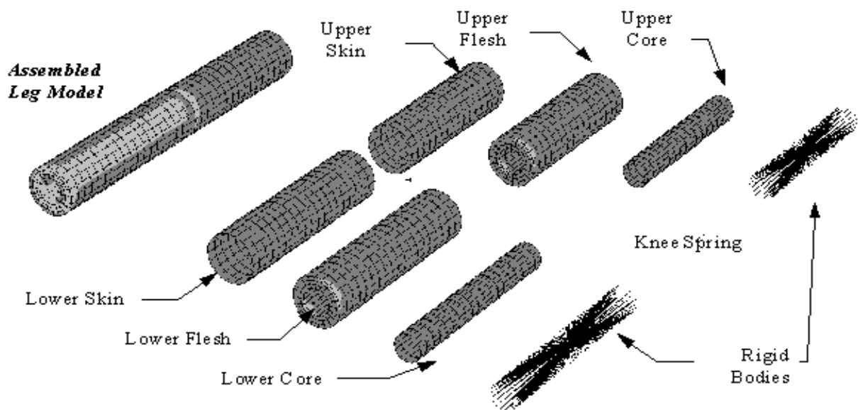
Figure 1: CAE Leg Impactor Model Construction
