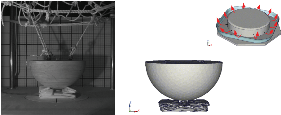
Figure 17: Test setup and corresponding finite element model
