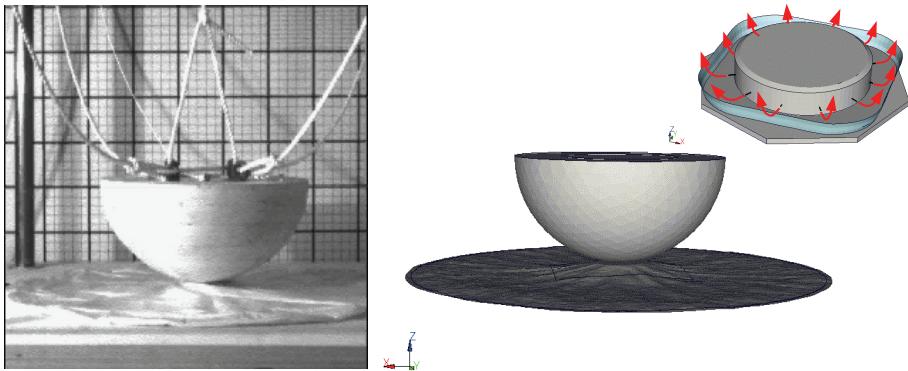
Figure 15: Test setup, corresponding airbag, impactor and deflator finite element model
