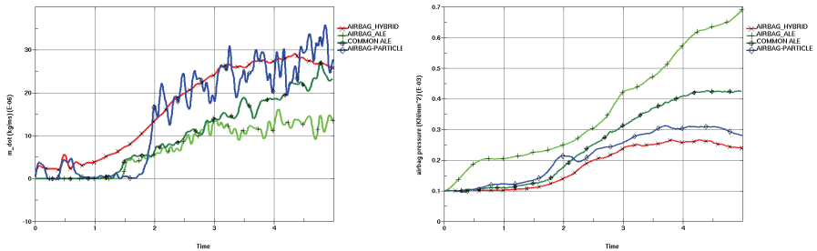
Figure 9: a) outgoing mass flux b) airbag pressure
