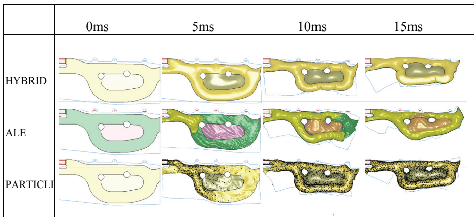
Figure 11: Multiple chamber airbag deployment study
