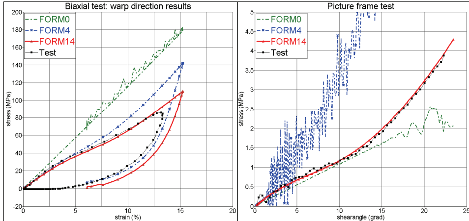
Figure 2: Biaxial tension and picture frame test
