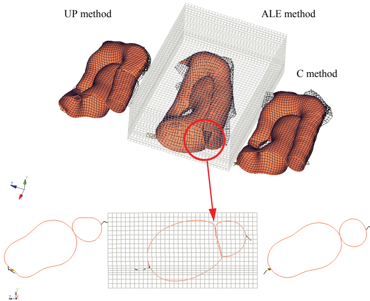
Figure 12: Detail of airbag chambers and cross sections at 10 ms
