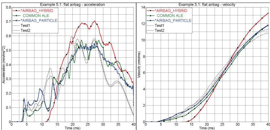
Figure 16: Acceleration and velocity of the semi-sphere compared to test data
