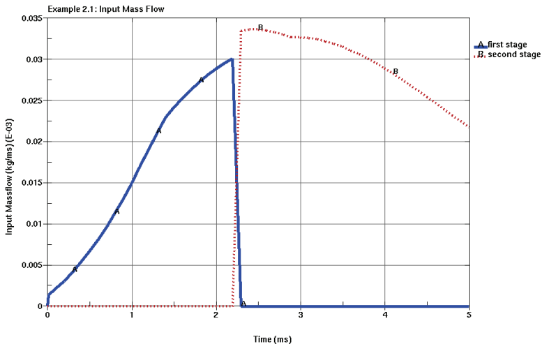
Figure 5: Separated mass flows for inflator
