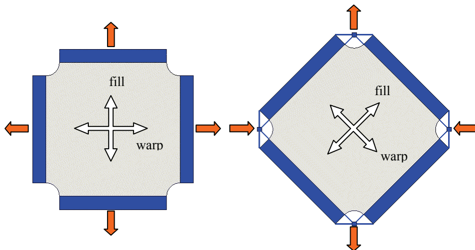
Figure 1: Biaxial tension and picture frame test
