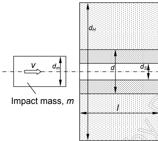
Figure 1: Interference fit with an impact mass
