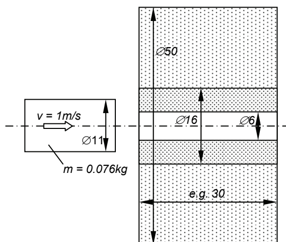
Figure 3: Model Geometry
