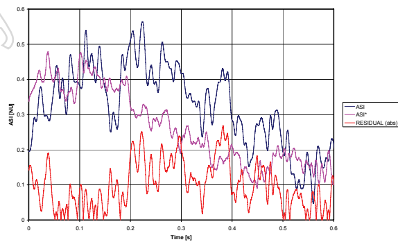
Figure7: device4 ASI curves
