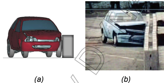
FIGURE 3: Crash test with a small car, (a) Finite Element simulation and (b) full-scale crash test.
