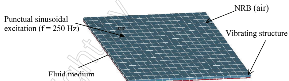
Figure 4: Vibrating plate model used in Kirchhoff method
