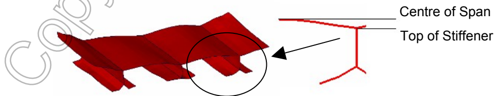
Figure 9: Structure Deformed due to Pressure Wave, showing relative deck heights
