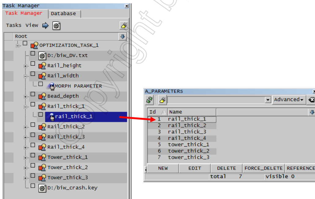
Figure 12: Connecting ANSA Parameters
