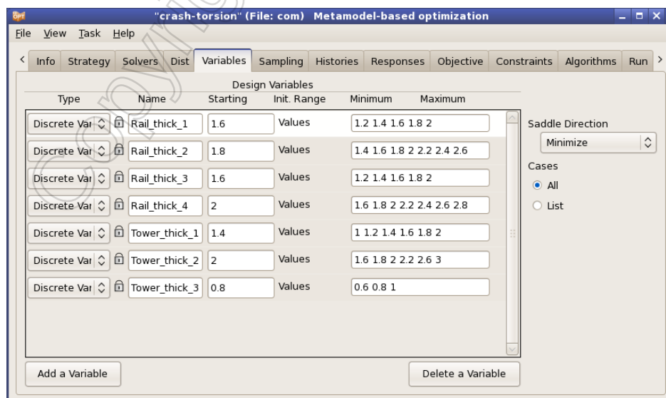
Fig. 21. The design variables in LS-OPT
