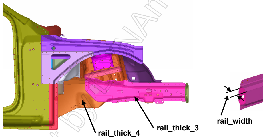
Figure 3: Design variables
