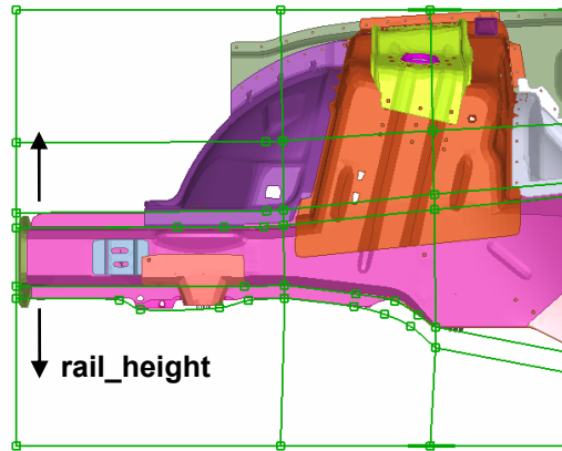
Figure 6: Rail initial shape
