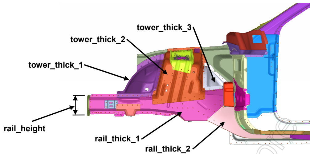
Figure 2: Design variables
