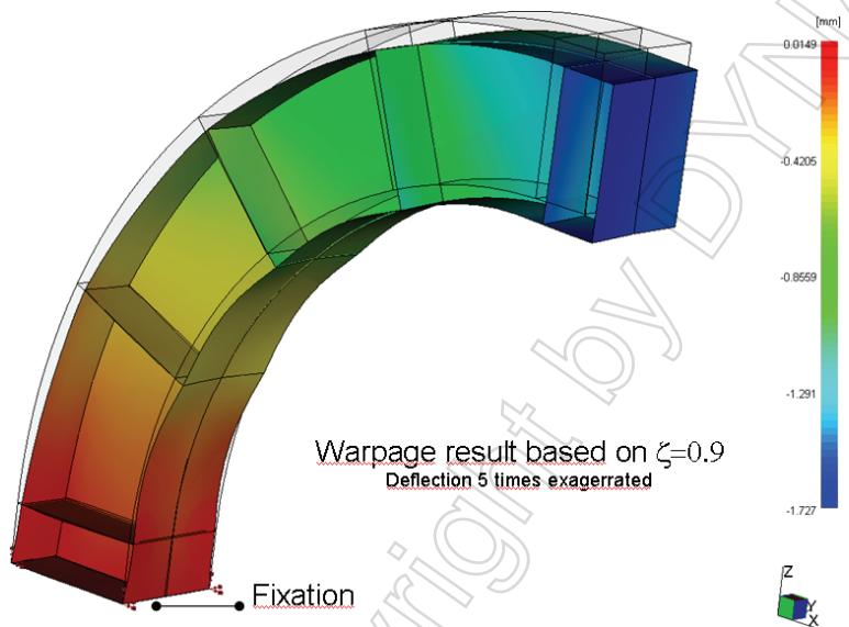
Figure 7: Warpage Simulation with Moldflow
