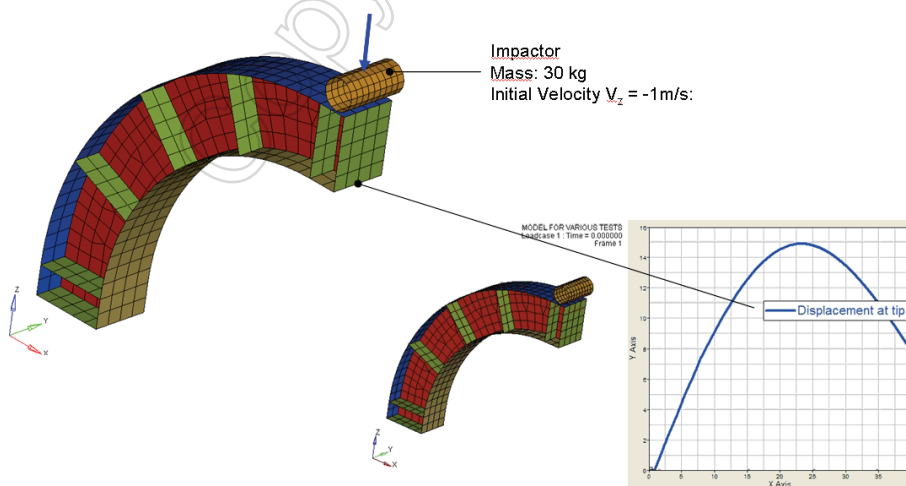
Figure 8: Impact Simulation with LS-Dyna, Impactor guided in z-direction
