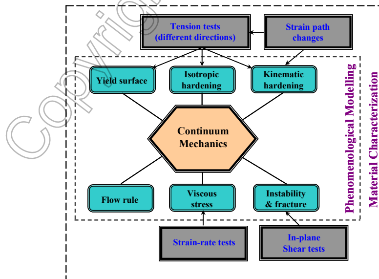
Figure 1. Identification of material parameters for the chosen constitutive model
