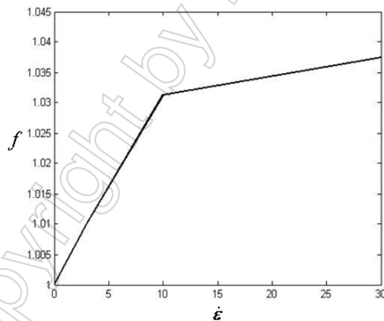
Figure 4: Strain rate effect
