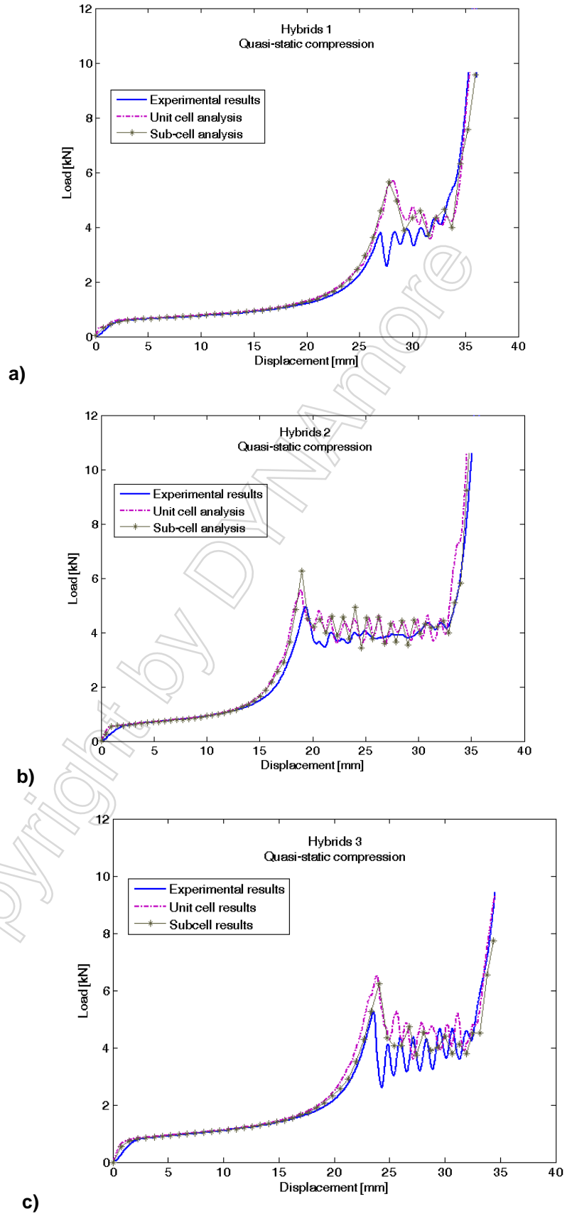
Figure 5: Force versus displacement curves - a) hybrids 1; b) hybrids 2; c) hybrids 3
