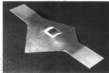
Figure 4: Tested Yoshida-specimen [8]
