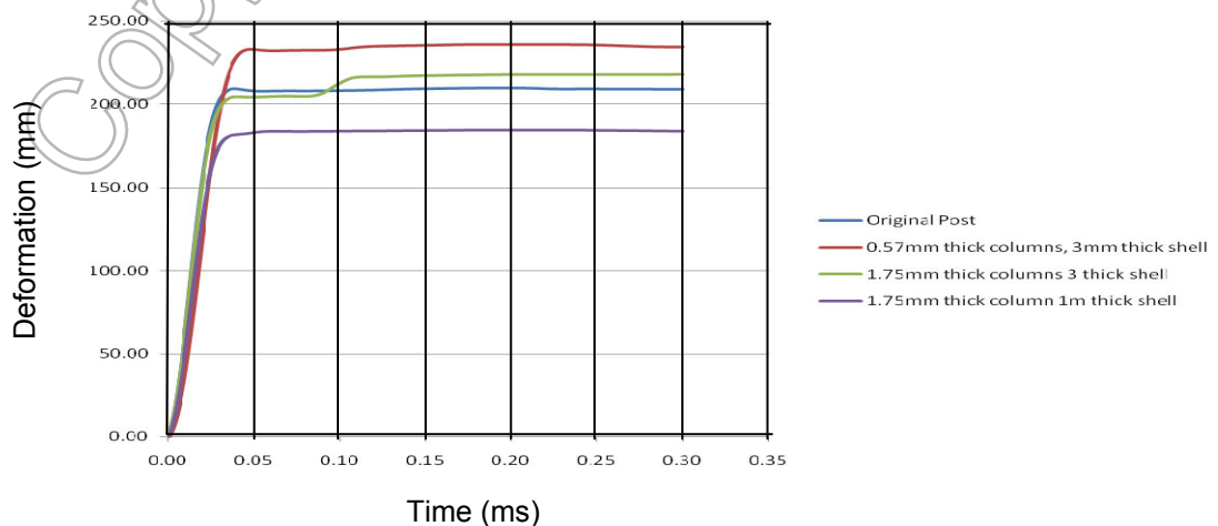
Figure 5: Deformation of the front-end.
