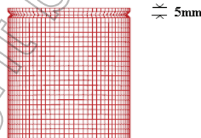
Figure 3: Crumple initiator positioned 5mm from the top of the tube.
