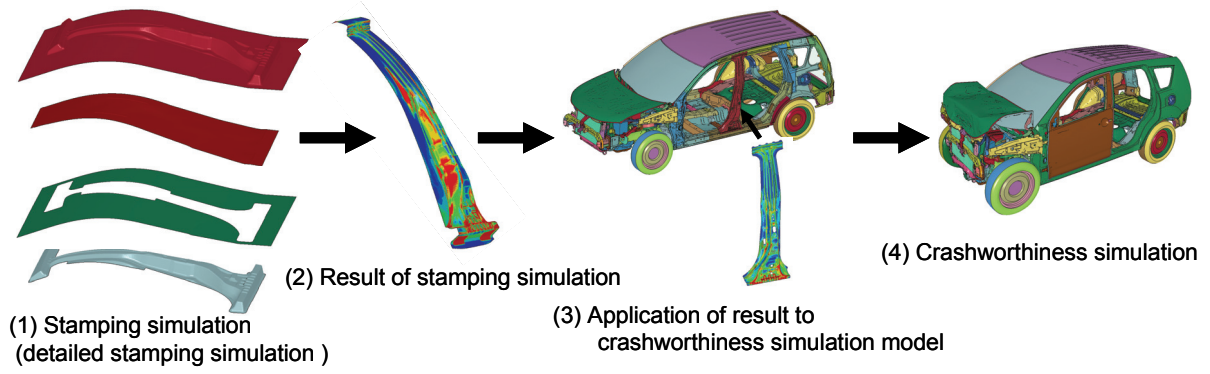
Fig. 1 Conventional process
