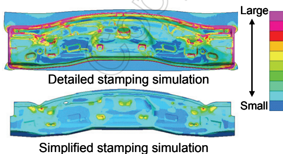
Fig. 3. Residual strain distribution.
