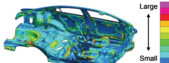
Fig.7 Residual strain distribution (example for parts in side impact simulation)
