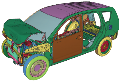
Fig.8 Vehicle deformation([1]Frontal impact)
