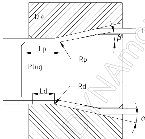
Figure 1: Sketch of conventional tube drawing with a floating plug
