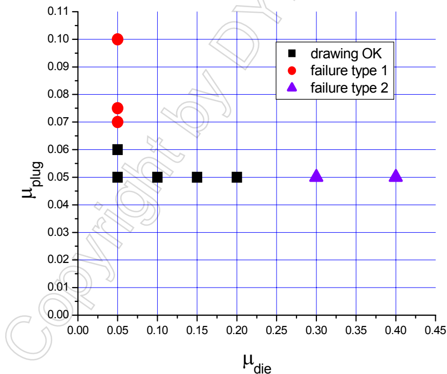
Figure 4: 2D FEM simulations of the tube drawing were carried out with the different combinations of \mu_{\text{die}} and \mu_{\text{plug}} shown.
