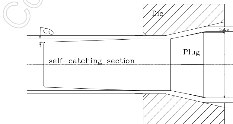
Figure 11: A self-catching plug. During start up the friction between the conical front end (self-catching section) and the tube wall will bring the plug into the right position in relation to the die
