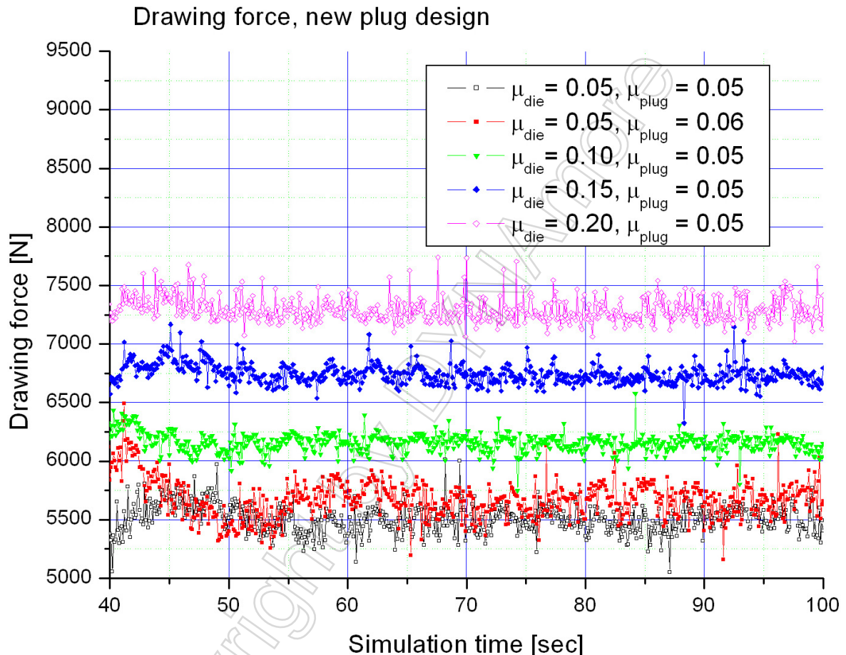
Figure 9: The tube drawing force with the new plug design for different combinations of the friction coefficients \mu_{\text{die}} and \mu_{\text{plug}}
