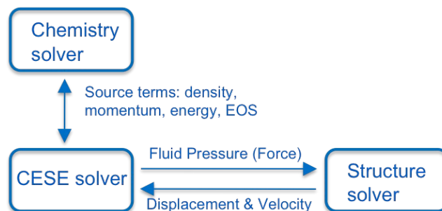
Figure 1 Interface data transfer
