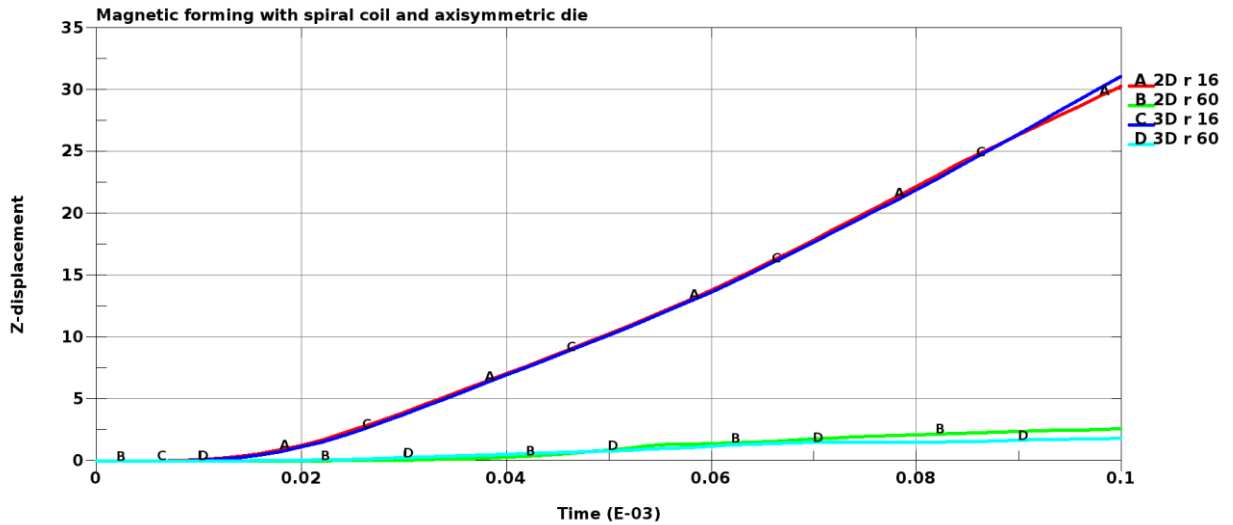
Figure 5: Comparison of displacements between 2D and 3D for two points along the workpiece's radius, one close to the center (radius = 16 mm), one further away (radius = 60 mm).
