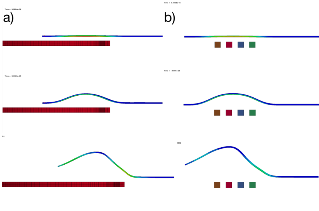
Figure 4: Lorentz force fringes at different times in a cross section of the workpiece. Comparison of the displacements between 3D, a) and 2D b).
