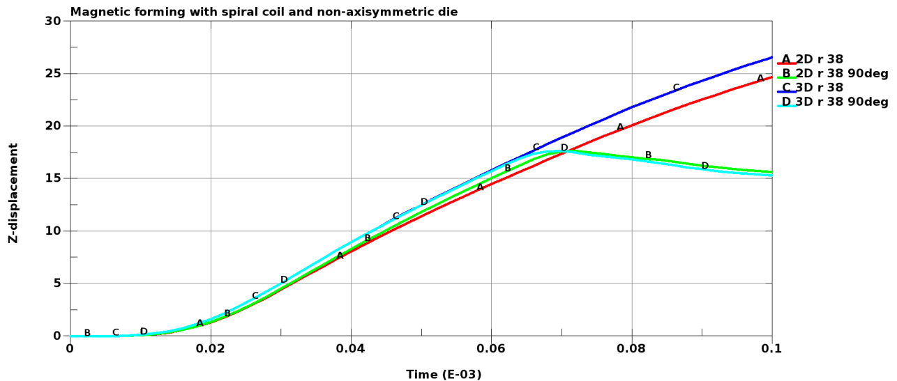
Figure 8: Comparison of displacements between 3D and 3D mixed with 2D for two points with the same radius but shifted by an angle of 90 degrees.
