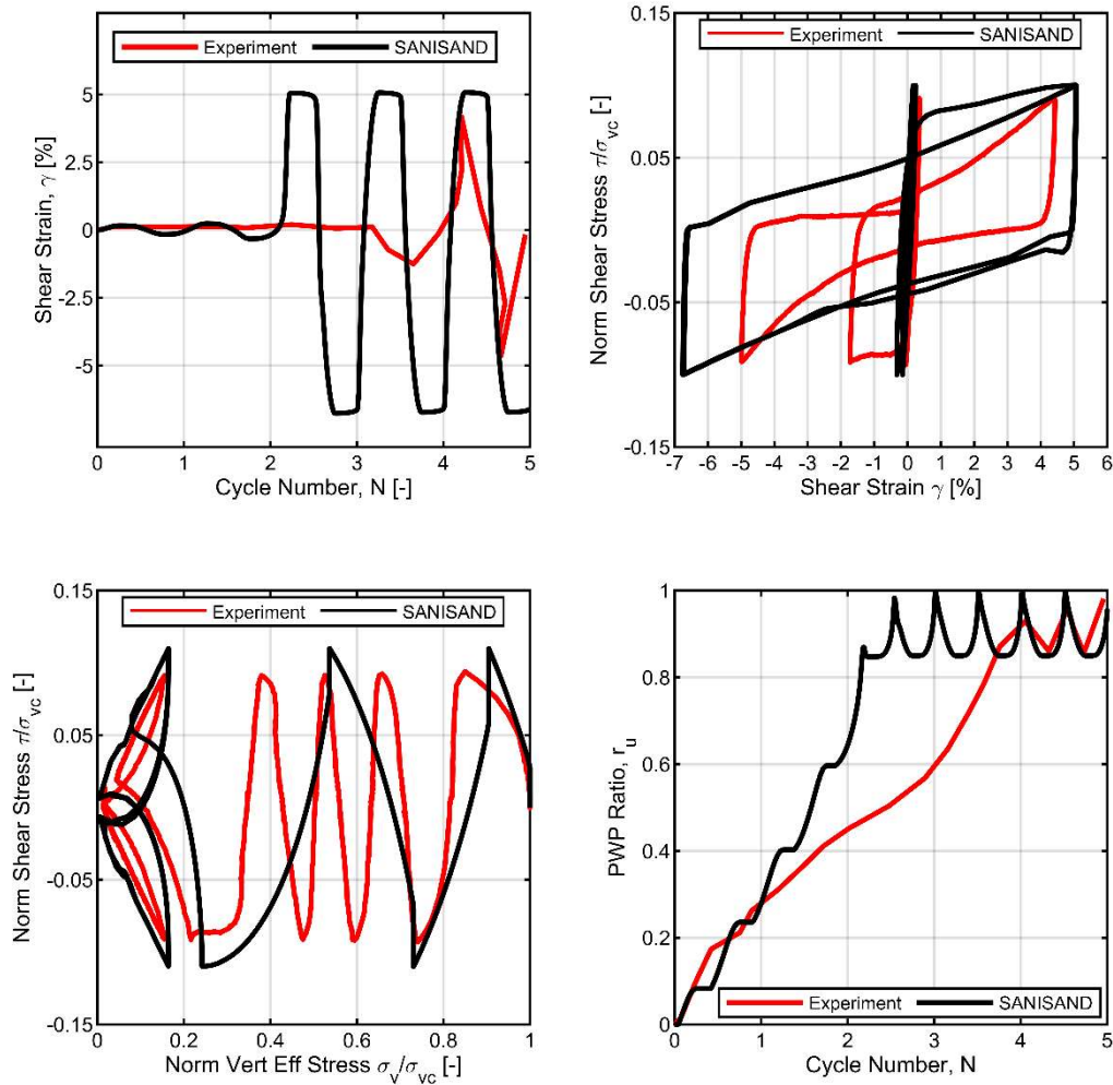
Fig.8: Comparison of physical and numerical element tests' results for Ottawa F-65 sand at a confining stress of 100 kPa
