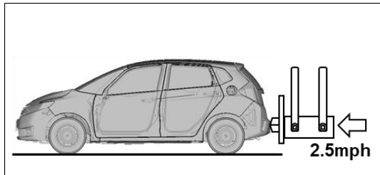
Fig.4-1: Overview of ECE42
