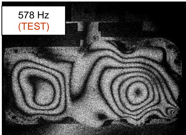
Figure 2 Mode Shape & Frequency from Test
