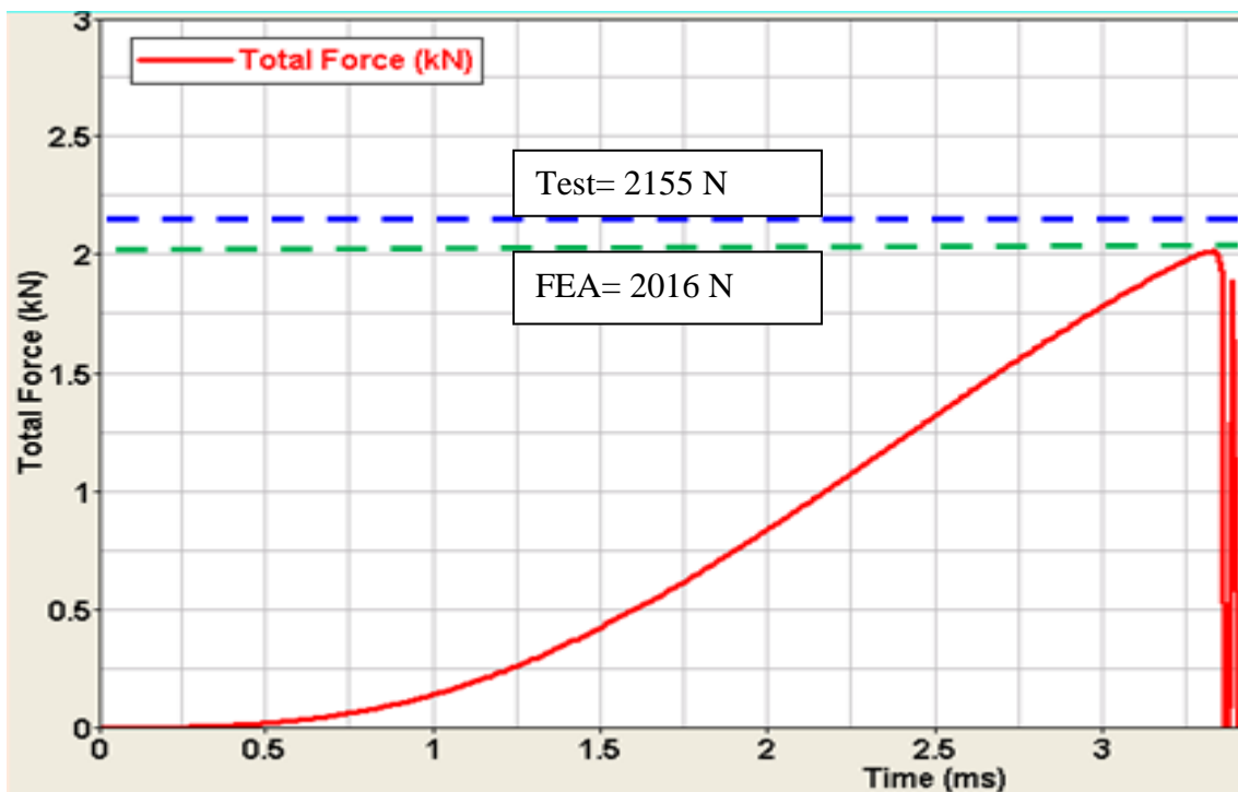
Figure 14 Comparison of Force from Test and CAE
