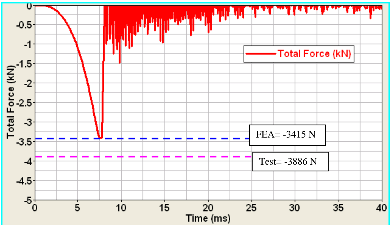
Figure 12 Comparison of Force from Test and CAE
