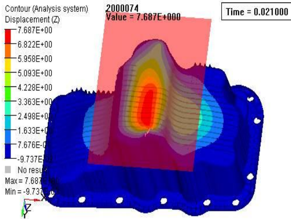
Figure 6 FEA Simulation of Crush Load
