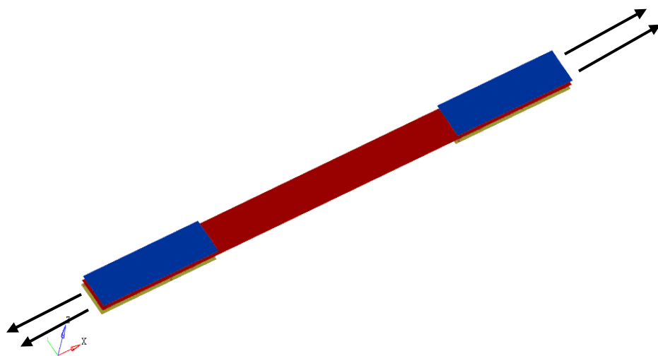
Figure 9 CFRT Laminate with (0-90-0)sym layup, tensile test along 90 0 Orientation
