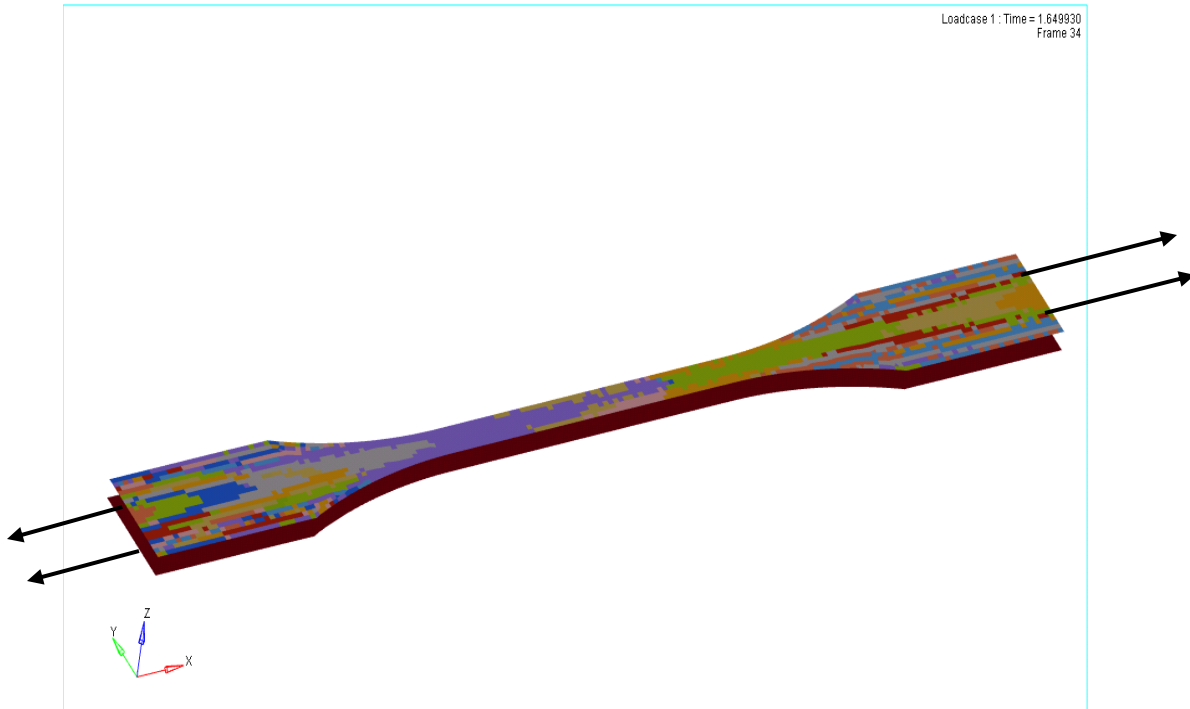
Figure 13 Over Molded SFRT (PA 6) over CFRT Laminate (0-90-0)sym, tensile test along 0°
