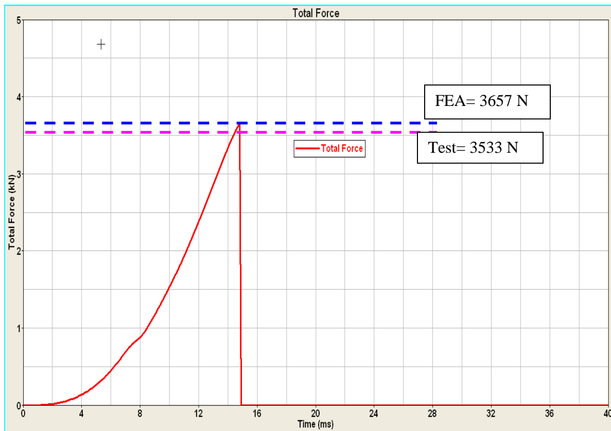
Figure 10 Comparison of Force from Test and CAE
