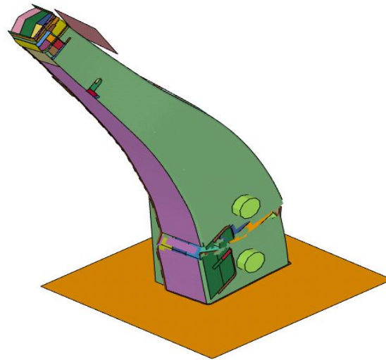
Figure 16 Failure after Push Test (FEA)
