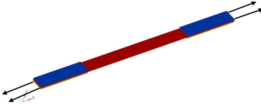
Figure 7 CFRT Laminate with (0-90-0)sym layup, tensile test along 0 0 Orientation
