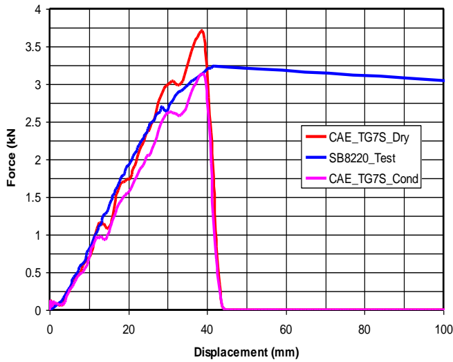
Figure 17 Force-Displacement Curve from Test & FEA
