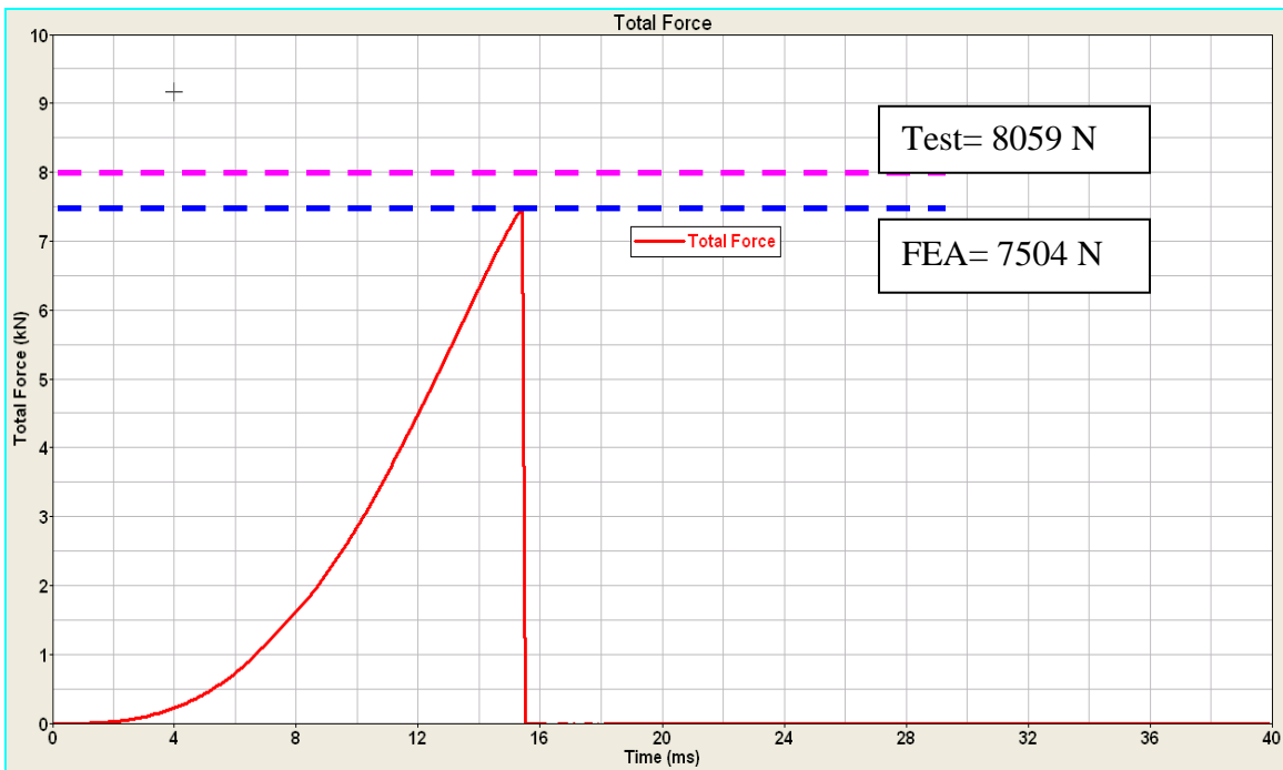
Figure 8 Comparison of Force from Test and CAE
