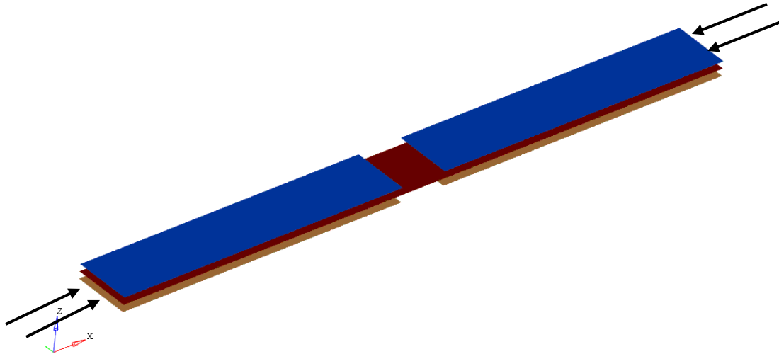
Figure 11 CFRT Laminate with (0-90-0)sym layup, compression along 0 0 Orientation
