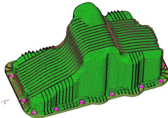
Figure 1 Plastic Oil Pan made of Ultramid A3WG7 (Glass Filled Polyamide 66)
