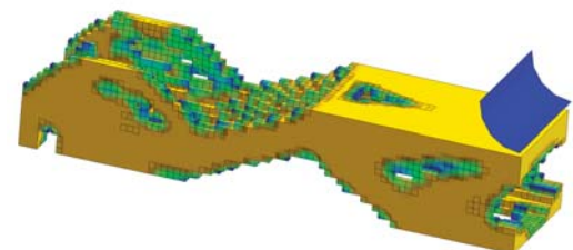
Topology Optimization
