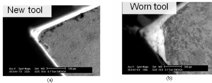
Figure 10. SEM images of (a) a new and (b) a worn tool.
