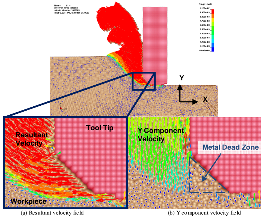
Figure 12. Velocity field at tool tip: Metal dead zone identification
