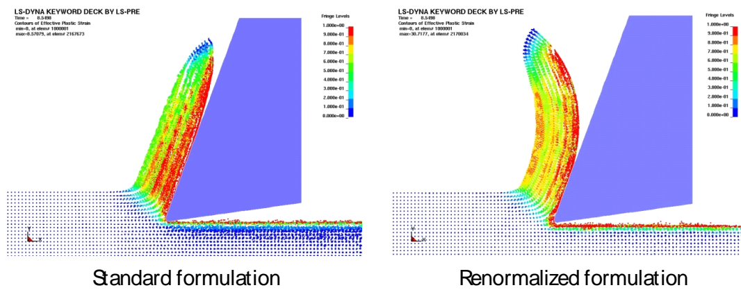
Figure 6. Standard/Renormalized SPH formulation in metal cutting
