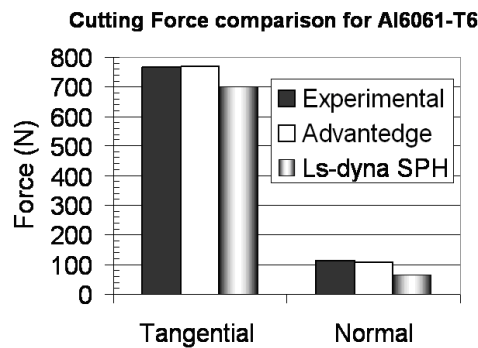
Figure 9. Al6061-T6 predicted cutting forces comparisons AdvantEdge/LS-DYNA
