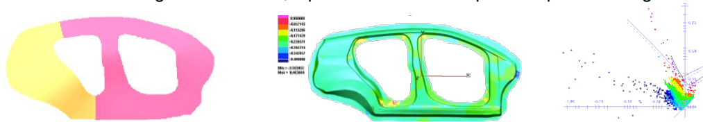
Figure 10: FSV body side outer incremental analysis results
